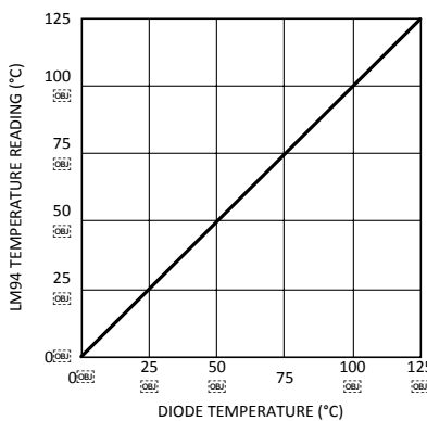
Figure 8. Thermal Diode Temperature vs. LM94 Temperature Reading
