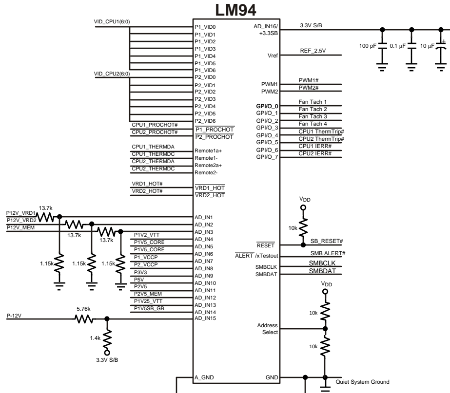
Figure 3. Recommended implementation without thermal diode connections
