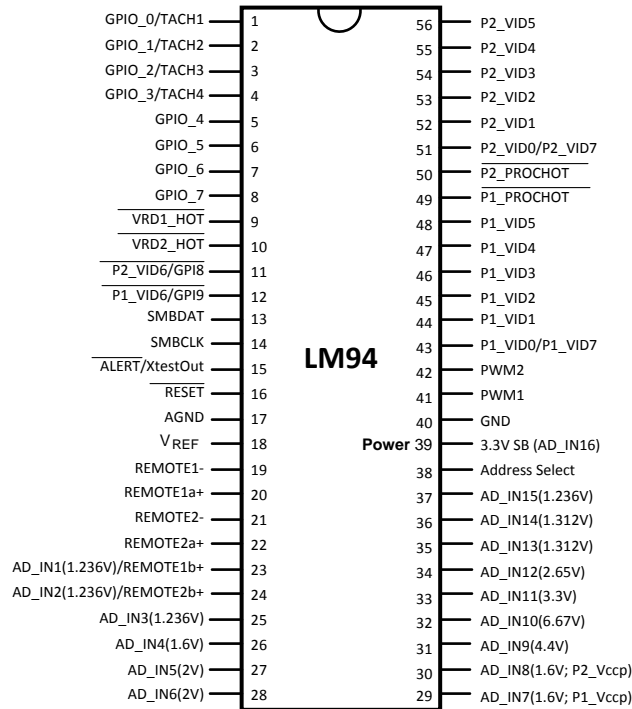
Figure 2. 56 Pin TSSOP NS Package MTD56
