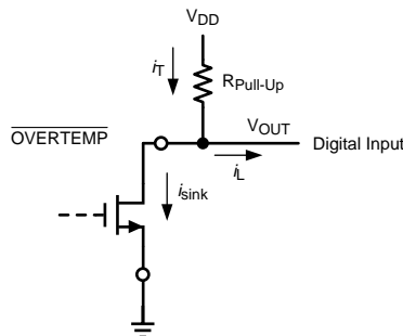
Figure 3. Determining the Pull-up Resistor Value
