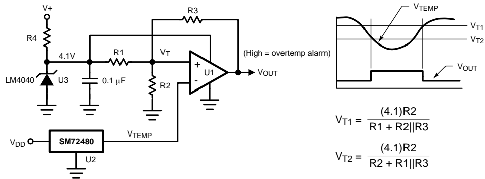
Figure 9. Celsius Temperature Switch
