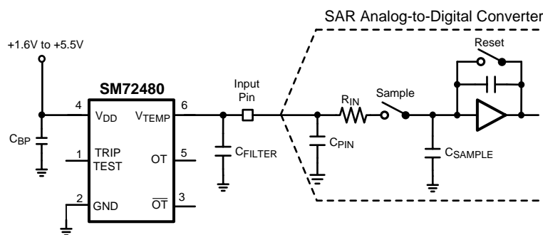
Figure 8. Suggested Connection to a Sampling Analog-to-Digital Converter Input Stage
