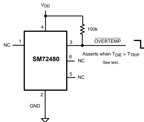
Figure 7. Temperature Switch Using Open-Drain Output
