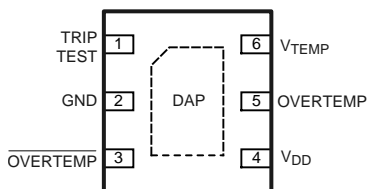
Figure 1. LLP-6 - Top View See NS Package Number SDB06A
