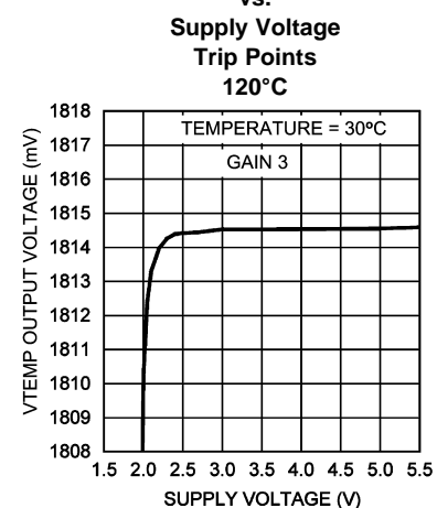
Line Regulation V TEMP vs. Supply Voltage
