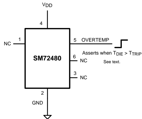
Figure 6. Temperature Switch Using Push-Pull Output
