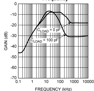
V TEMP Supply-Noise Rejection vs. Frequency
