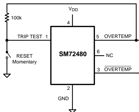
Figure 11. Latch Circuit using OVERTEMP Output
