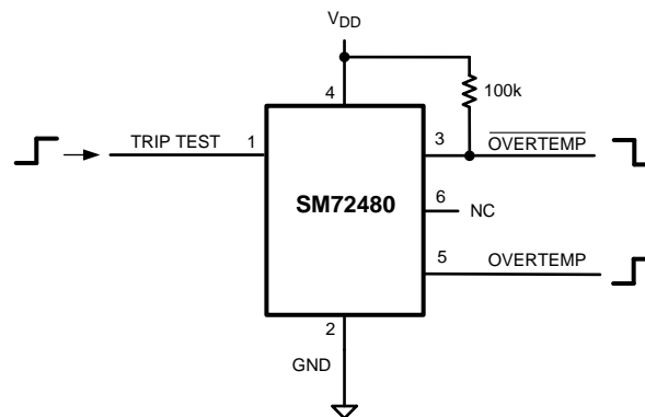
Figure 10. TRIP TEST Digital Output Test Circuit
