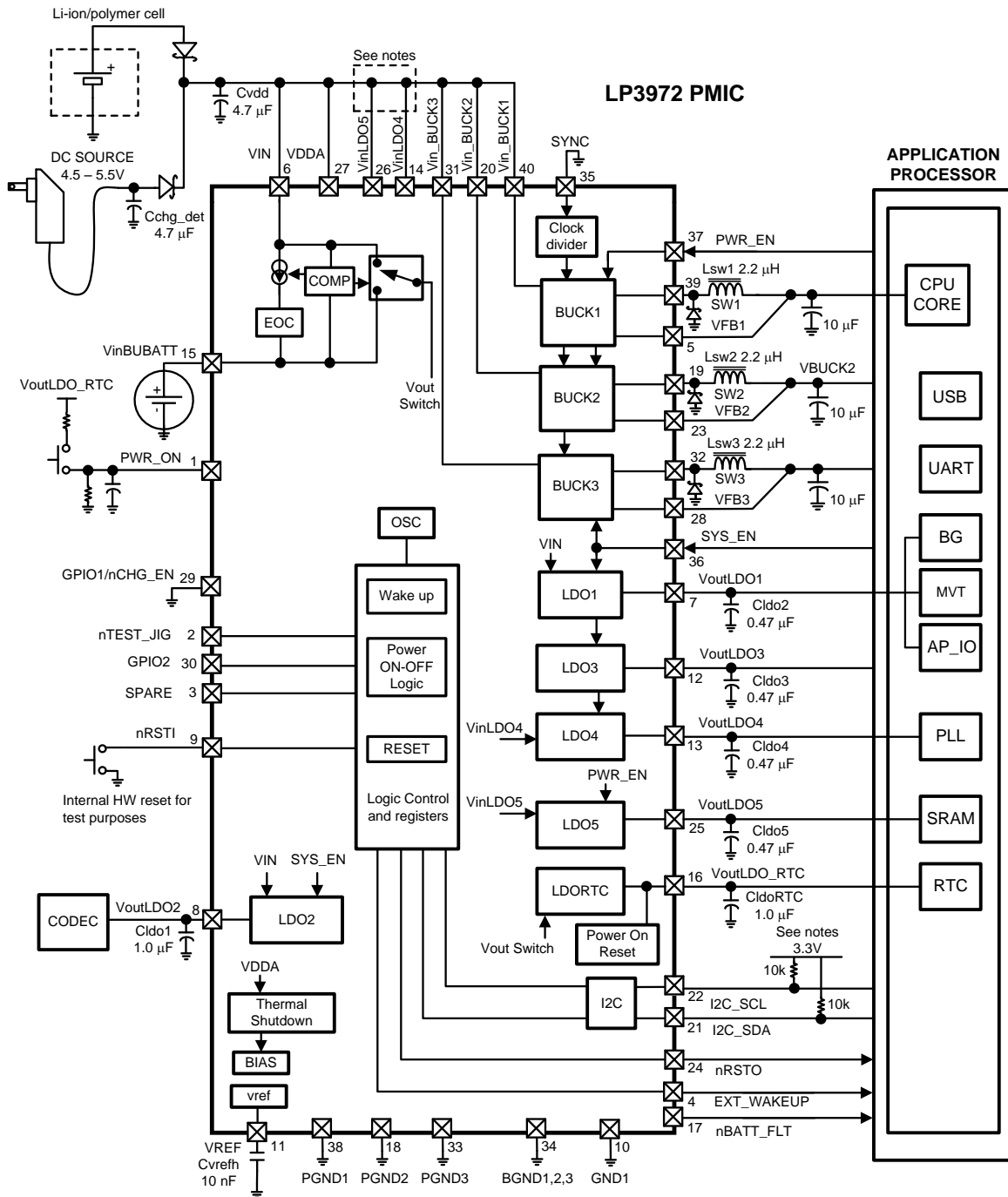
Figure 2. Application Circuit
