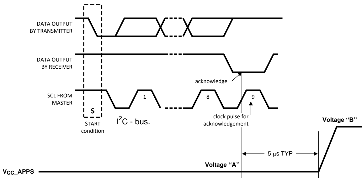
Figure 23. I²C DVM Timing for VCC_APPS (Buck1)
