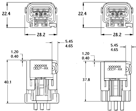
Sealed Assembly
